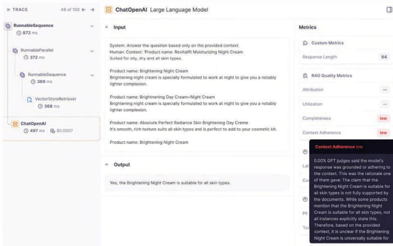
Fig 7.25: Context adherence explanation in Galileo GenAI Studio
