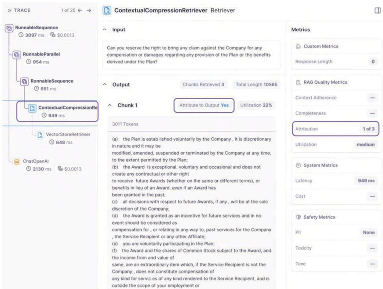
Fig 4.4.11: Total attributed chunks from the reranker and then what is each chunk's attribution
